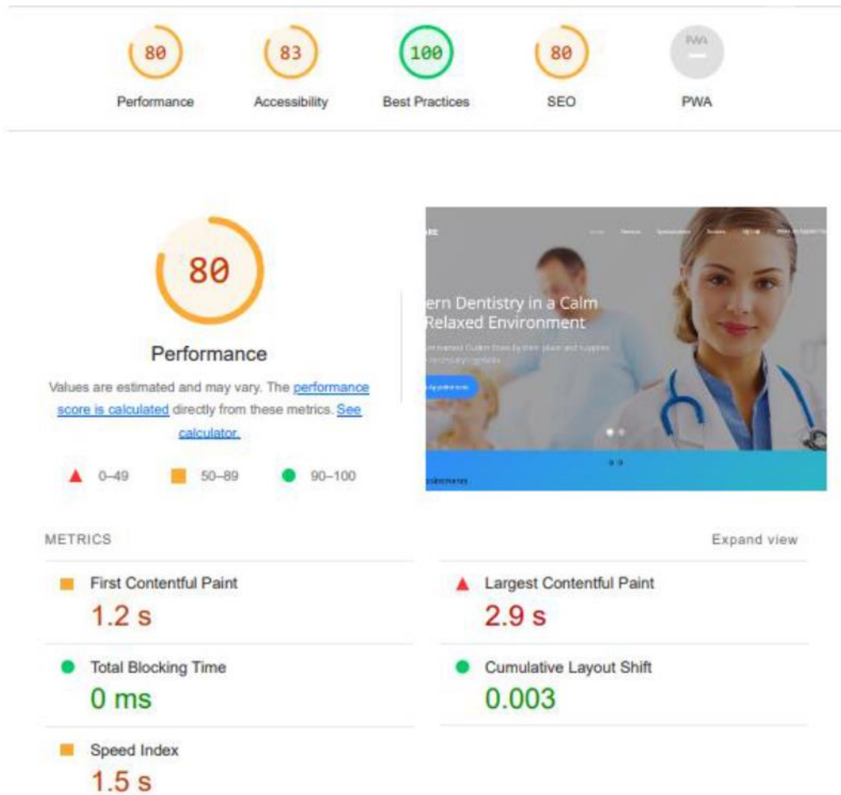
Figure.5.11 google lighthouse test
